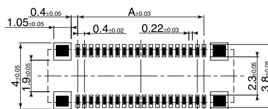
Socket (With Shield)
